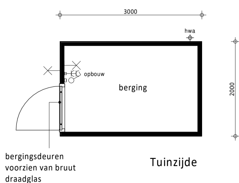
Plattegrond (type 2)
