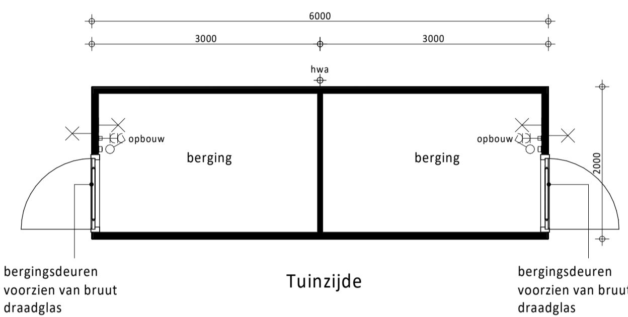
Plattegrond (type 1)
